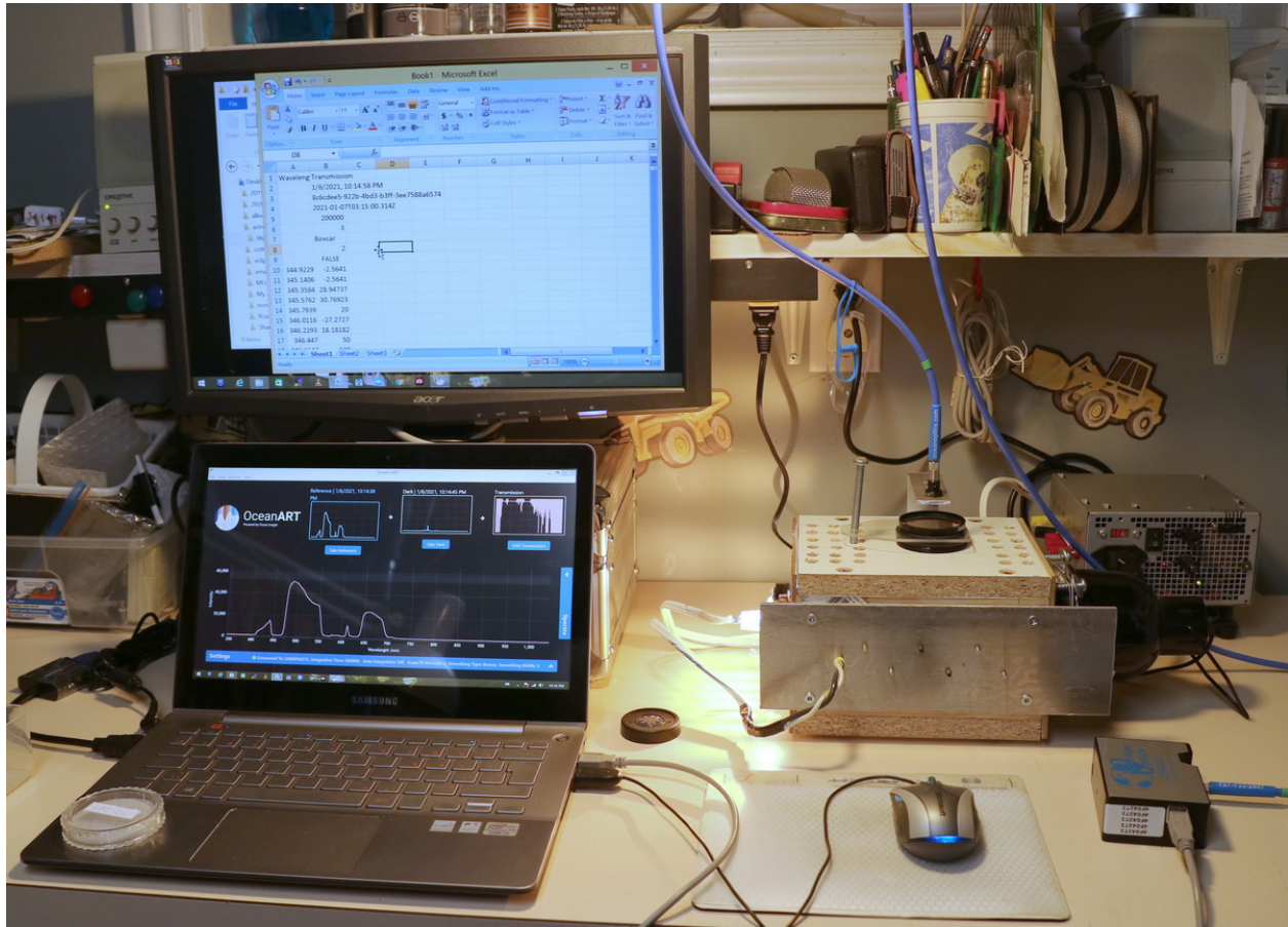
Figure D-1 Typical Setup for Filter Spectrum Measurement
