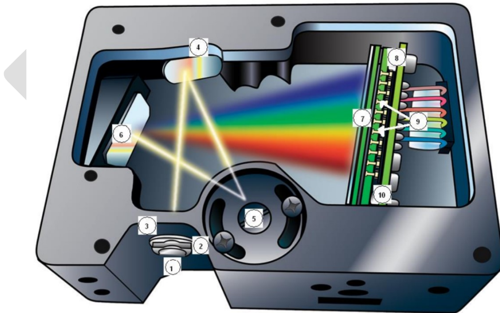
(1. SMA905 connector, 2. slit, 3. filter, 4. collimating mirror, 5. grating, 6. focusing mirror, 7. L4 detector collecting lens, 8. detector, 9. OFLV filters, 10. UV4 detector upgrade)
