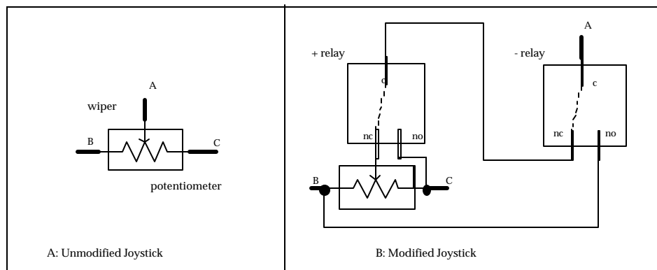
Figure 4.3 - Joystick Modification
