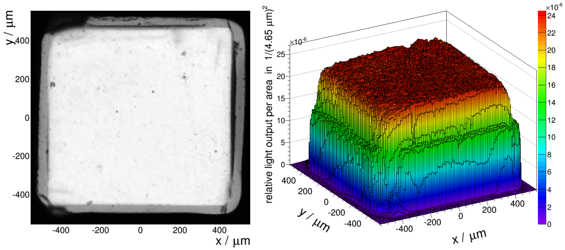
Figure 4.10: Left: Image of the end surface of the square multicladd scintillating fibre at a distance of approx. 10\mu\text{m} to the camera sensor. The image is corrected for dark noise and signal fluctuations (cf. section 4.2). Right: Relative light output per camera pixel (area: (4.65\mu\text{m})^2 ) given by the pixels' signal values divided by the integrated signal over all pixels. The light output is distributed rather homogeneously across the fibre surface.
