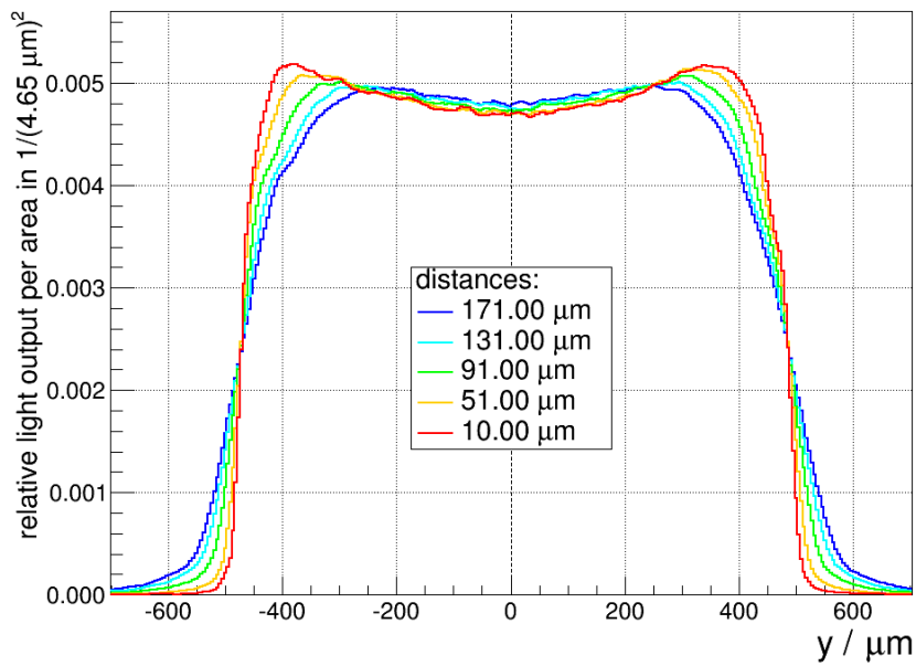
Figure 4.15: Light output profile through the centre of the round multicladd fibre measured with a camera sensor at varying distances towards the fibre end (pixel size: (4.65 \mu\text{m})^2 ). Each graph shows the signal values along the central pixel array in y -direction ( x = 0 \mu\text{m} = \text{const} , see fig. 4.9) normalised to the integral over the respective profile. For a better comparison the uncertainties are not shown and the profiles are slightly smoothed. The profile maxima at the fibre edges decrease for larger distances and the profile assumes a more Gaussian trend with a small dip at the centre. The shown widening of the profile with larger distances is more rigorous than in the case of the singleclad fibre (fig. 4.14).
