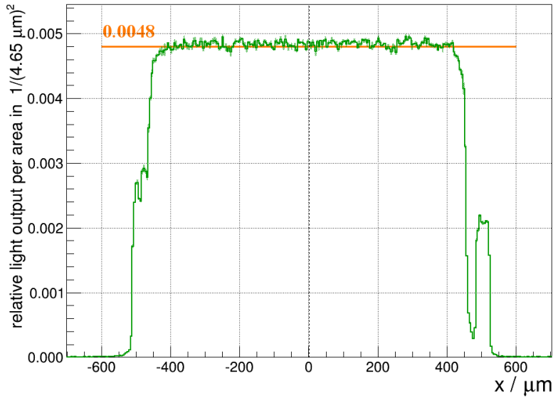
Figure 4.13: Light output profile through the centre of the square multiclad fibre measured with a camera sensor approx. 10\ \mu\text{m} away from the fibre end (pixel size: (4.65\ \mu\text{m})^2 ). The plot shows the signal values along the central pixel array in x-direction ( y = 0\ \mu\text{m} = \text{const} ; see fig. 4.10) normalised to the integral over the profile. The light is very evenly spread across the fibre profile. The peak at x \approx 500\ \mu\text{m} results from damage inflicted on the cladding during the fibre preparation.
