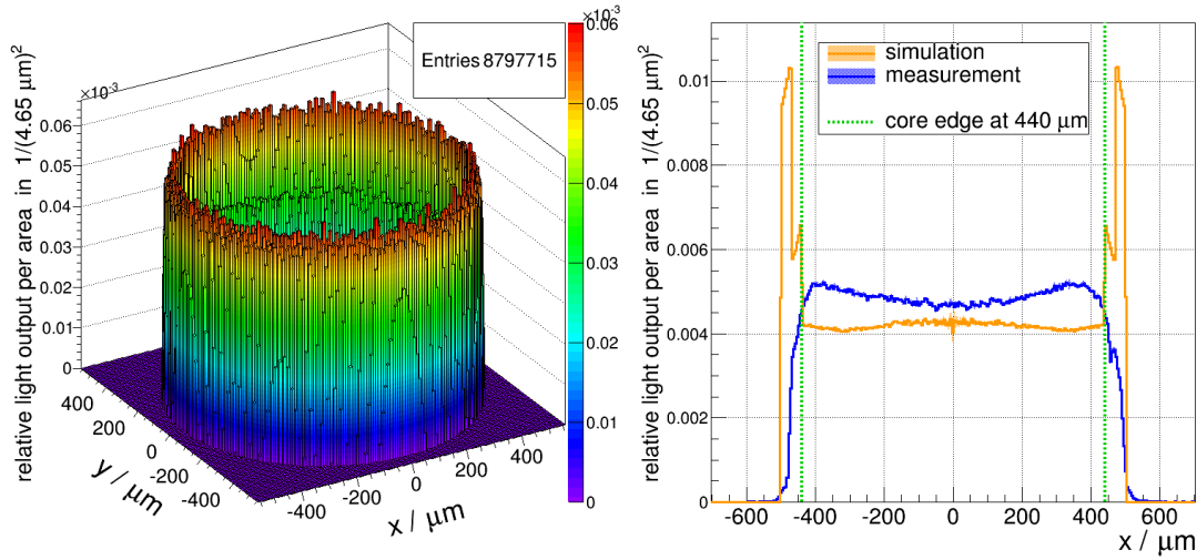
Figure 5.4: Left: Simulated spatial distribution of the light output (photon count) per area relative to the total photon count for the round multicladd WLS fibre (at a distance of 10 \mu\text{m} towards the fibre end surface). Right: The corresponding light output profile through the fibre centre for the initial simulation (orange; cf. fig. 5.3) and measurement (blue; see fig. 4.12). It shows that the profiles do not match. For the simulation, the fibre claddings feature a much higher light output per area than the fibre core.
