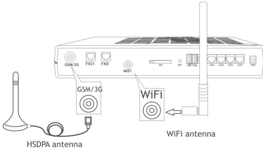
Figure 6: Antenna attachment
